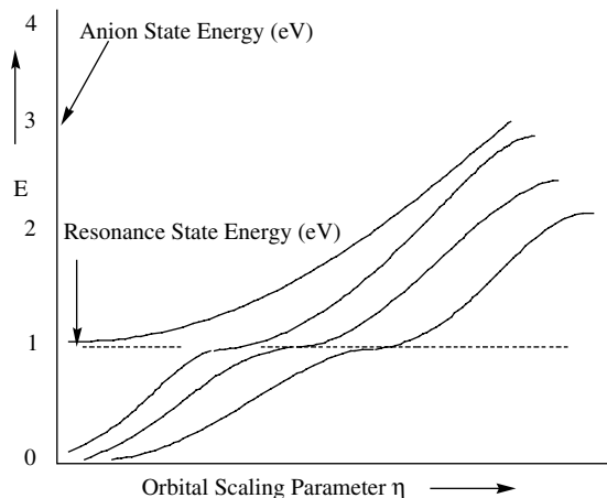
764 Fig. 17.1. Plots of the EOM-EA eigenvalues for several anion states vs. the orbital scaling parameter \eta . Note the 765 avoided crossing of state energies near 1 eV.
